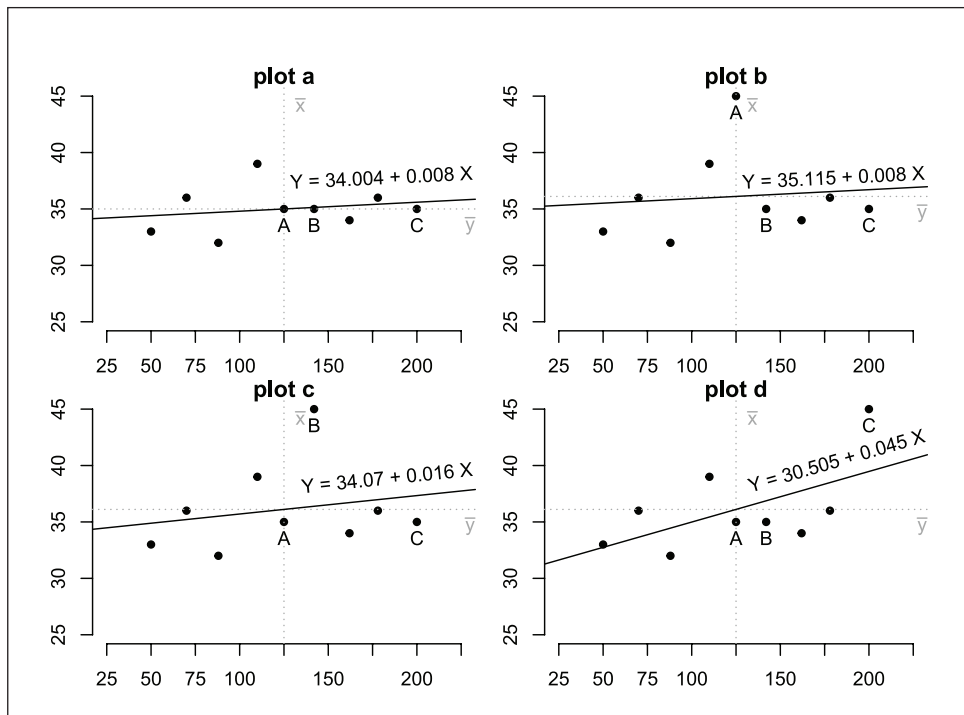
Figure 2: Impact of an individual having extremely large or low coordinate on the Y axis, on the regression slope, as a function of its coordinate on the X axis.
