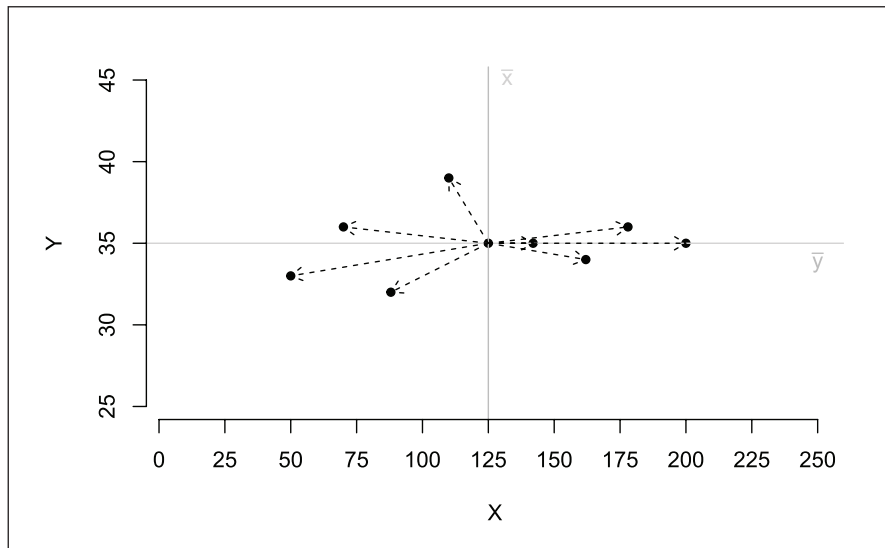
Figure 1: Illustration of individual slopes of lines linking all data of the scatter dot and the G-point.
